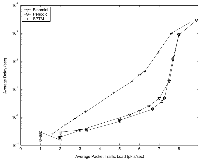
Figure 3.13. Average delay vs. average load for the S-MAC protocol under different packet traffic patterns ( log )
