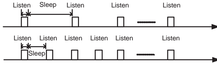
Figure 2.4. DSMAC duty cycle doubling [31]
