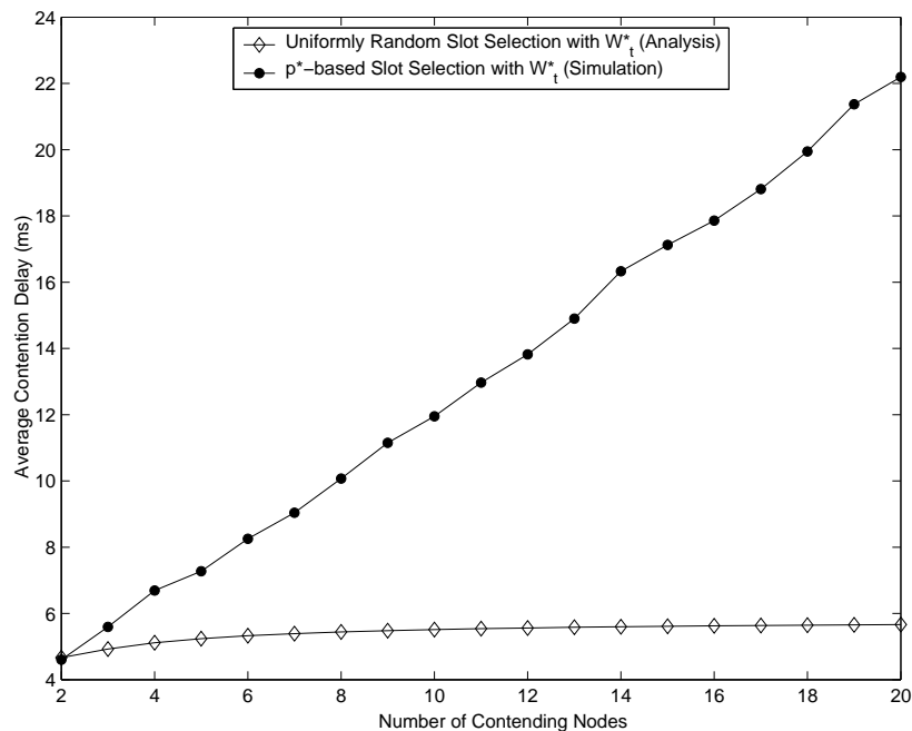
Figure 4.19. Average contention delay results for different slot selection methods for CW size of W_t^*
