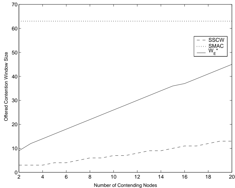
Figure 4.11. The offered contention window sizes by SSCW, S-MAC, W_E^*
