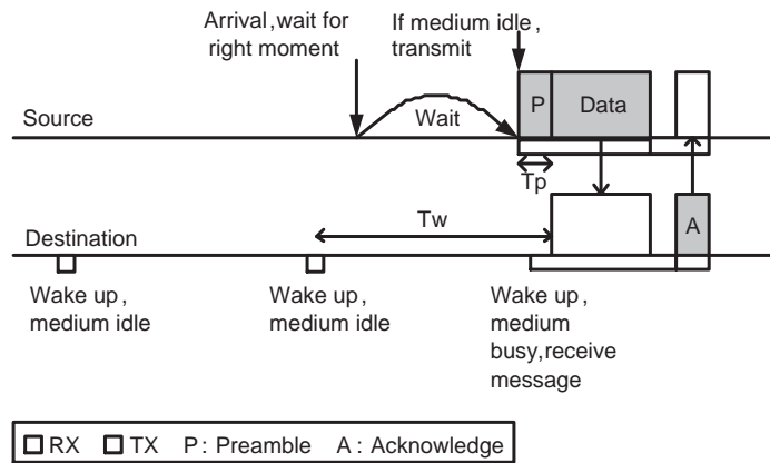
Figure 2.2. WiseMAC Concept [23]
